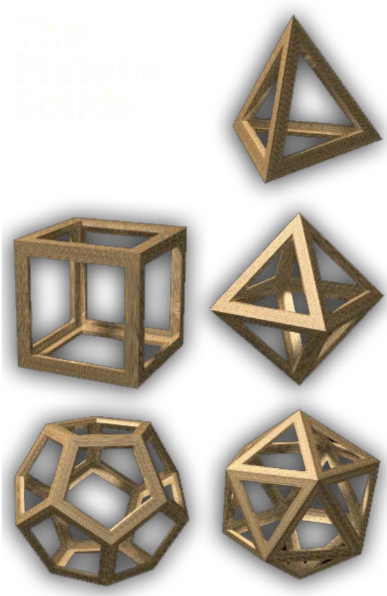
Platonic Solids
